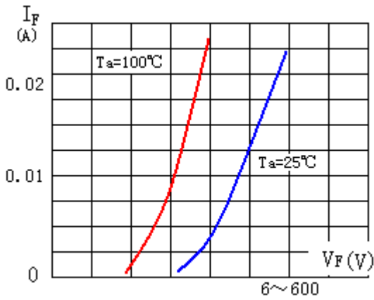
Forward Characteristics
